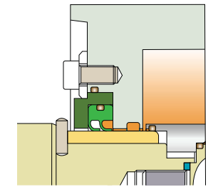
Lip Seal
